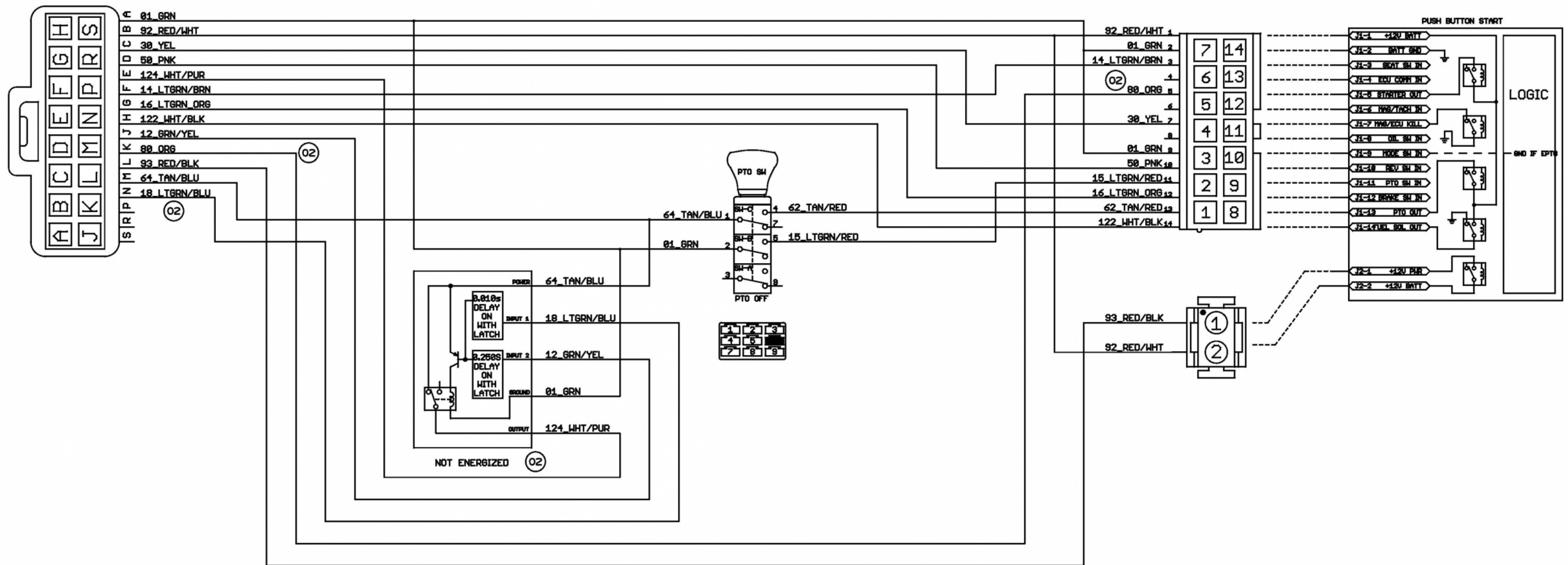
MAIN HARNESS CONNECTION 1
