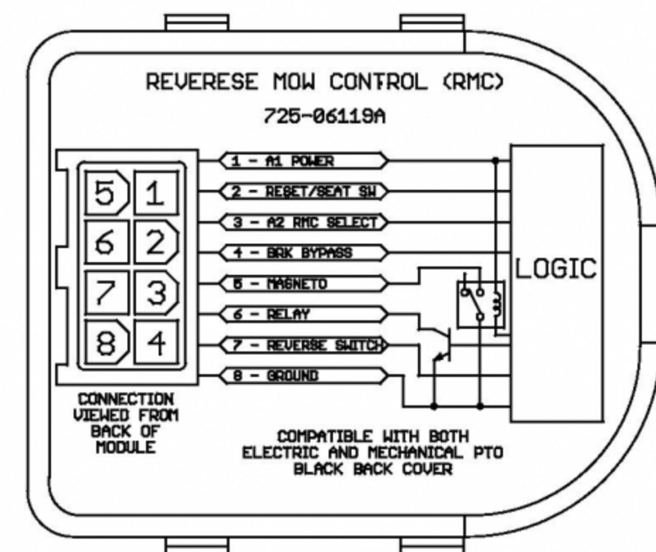
RMC CONNECTOR
