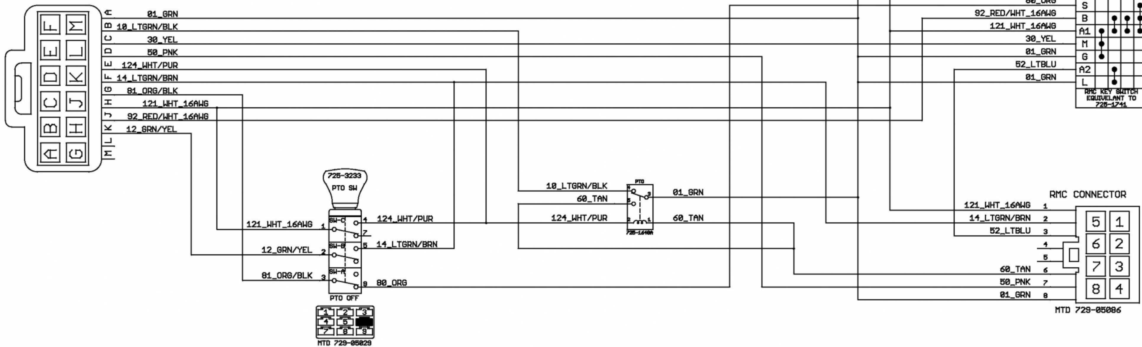
MAIN HARNESS CONNECTION 1 MTD 729-05138
