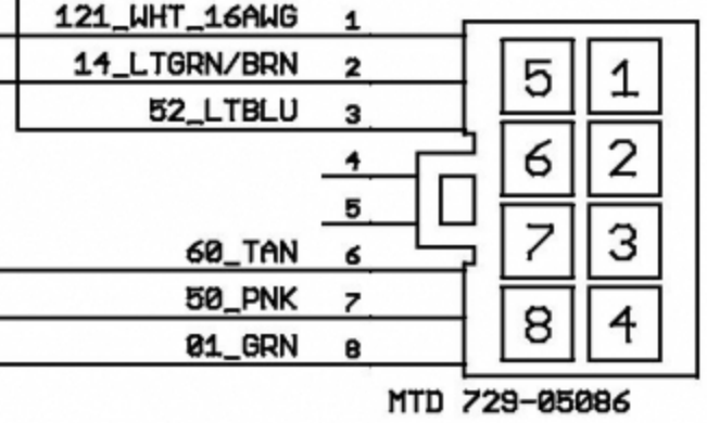
RMC CONNECTOR
