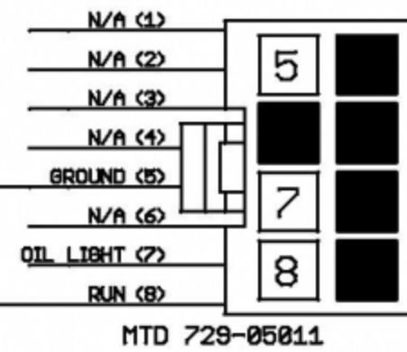
HOUR METER CONNECTOR
