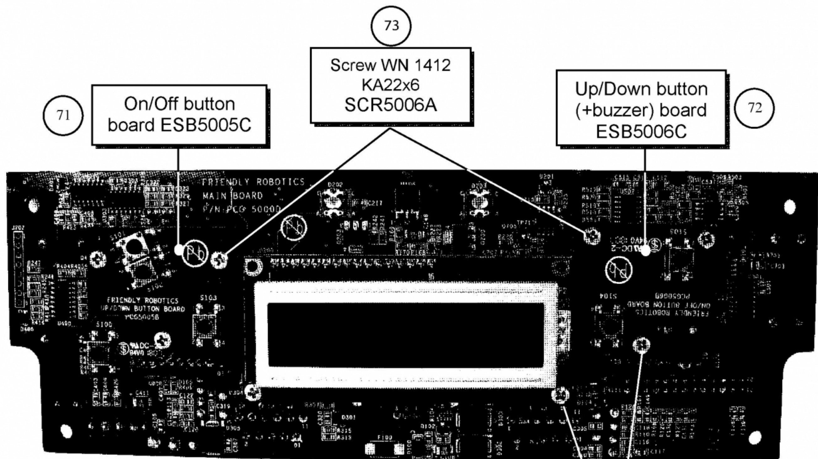
Main Board Top View
