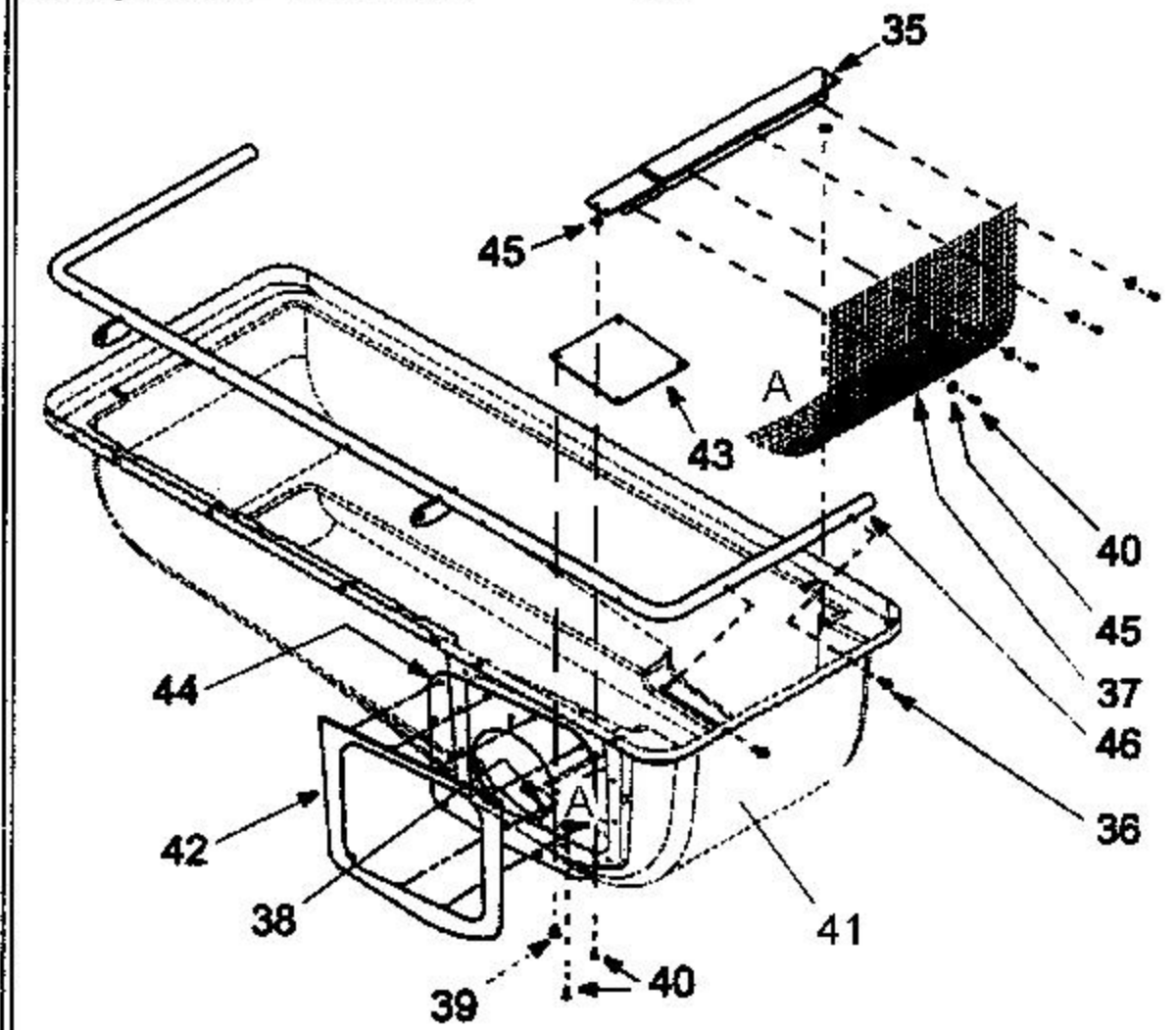
Components of Cover Assembly pn # 664-04018 Ref 4
