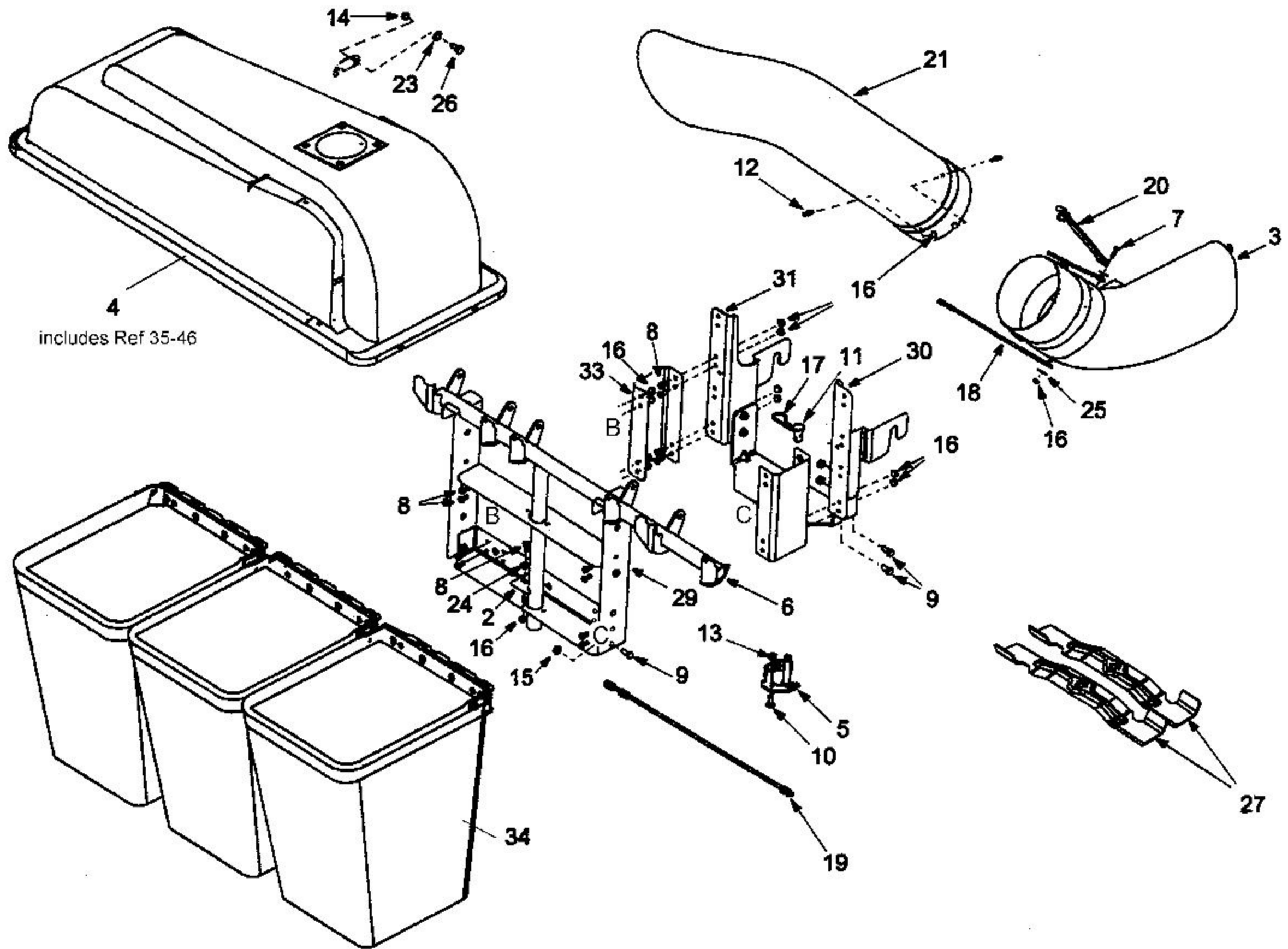
Components of Cover Assembly pn # 664-04018 Ref 4
