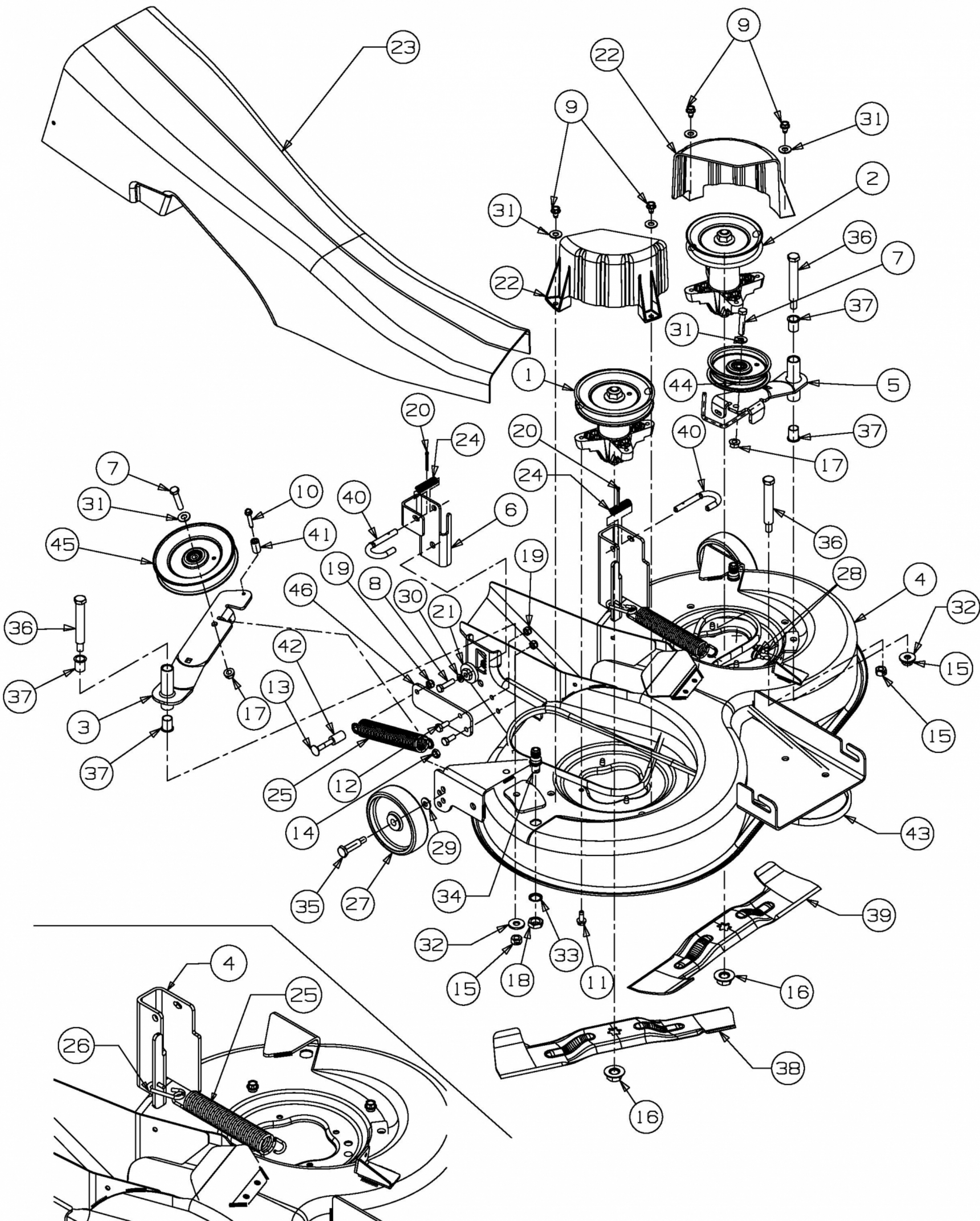
Installation of spring / Federmontage
