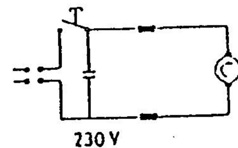
SCHEMA ELECTRIC
